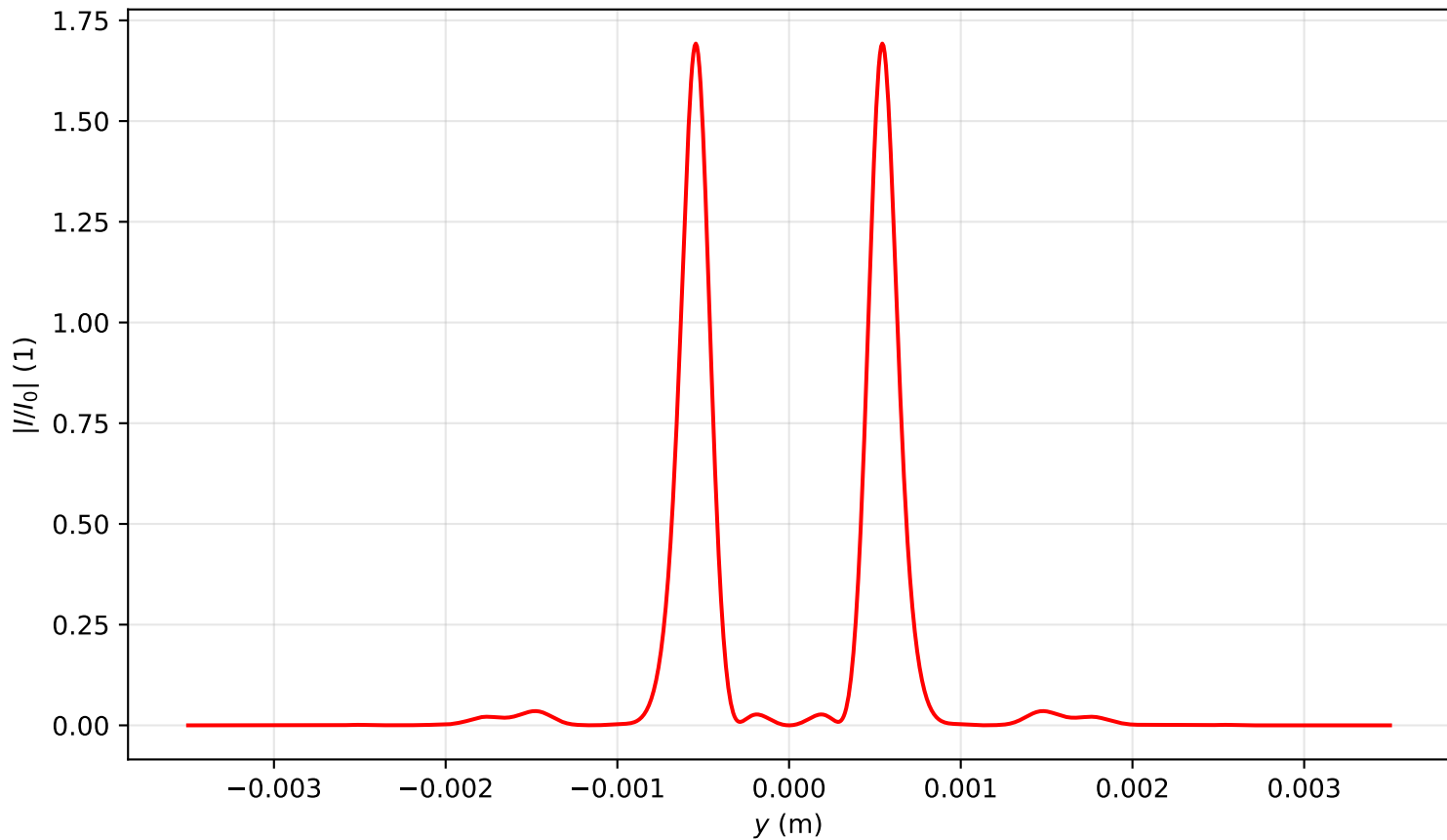
Intensity profile I(x=0, y, z=1.353)/I_0 , P_{in}=9.0P_{cr} , artificial time
